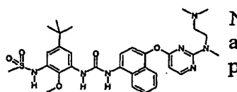
N-{5-tert-Butyl-3-[3-(4-{2-[(2-dimethylamino-ethyl)-methylamino]-pyrimidin-4-yloxy}-naphthalen-1-yl)-ureido]-2-methoxy-phenyl}-methanesulfonamide;
